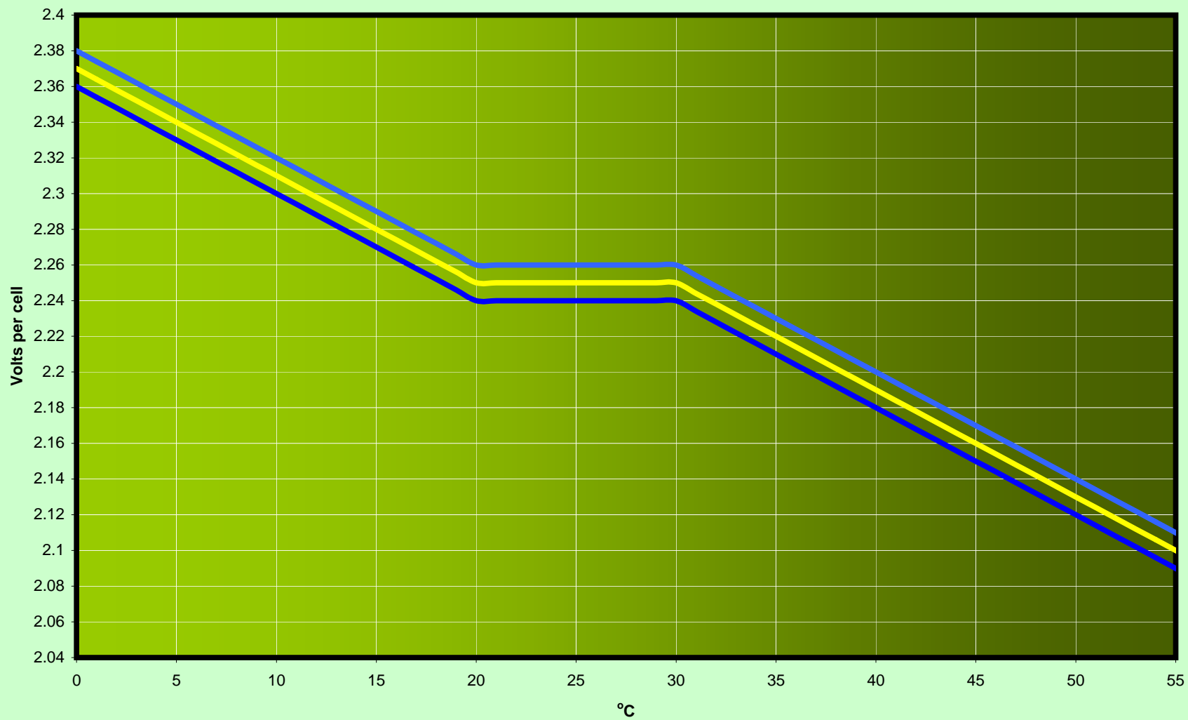
Enerlyte Float voltage vs Temperature
