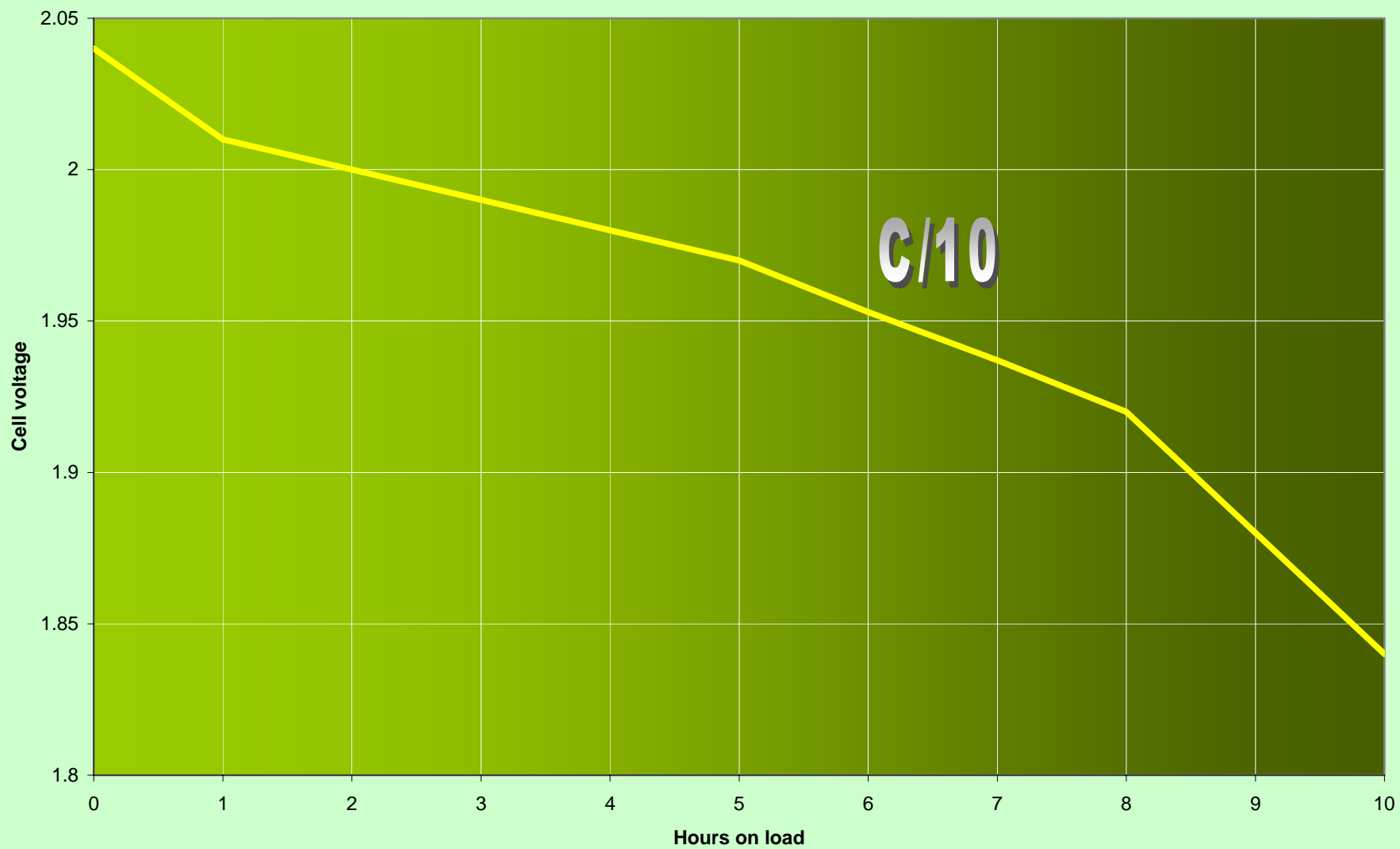
Enerlyte typical discharge curve
