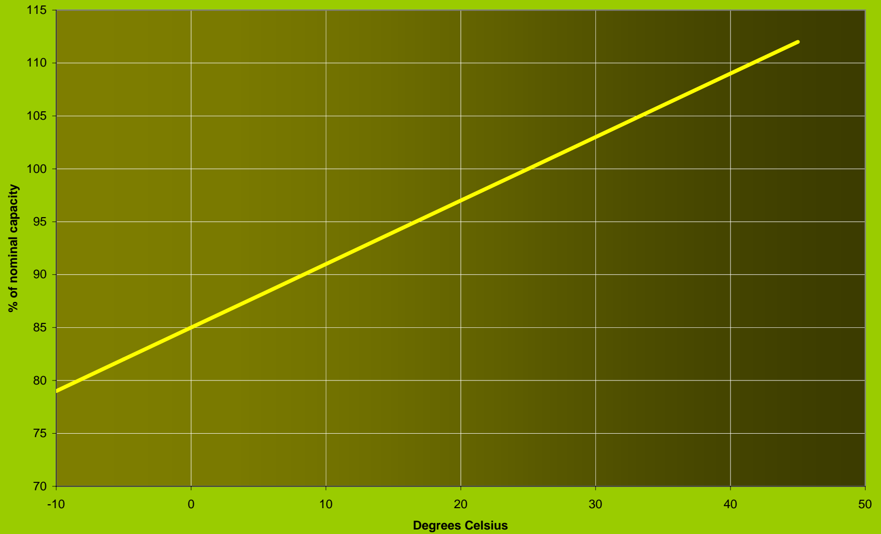
Railgel capacity vs temperature
