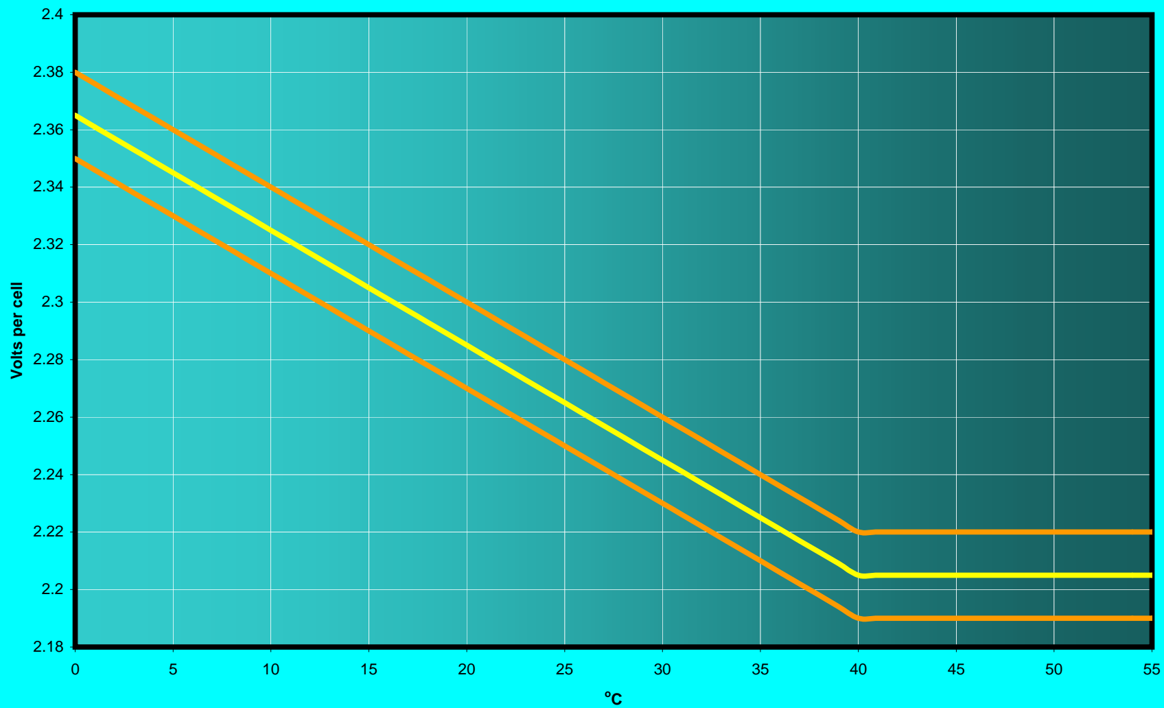
Marinegel Float voltage vs Temperature
