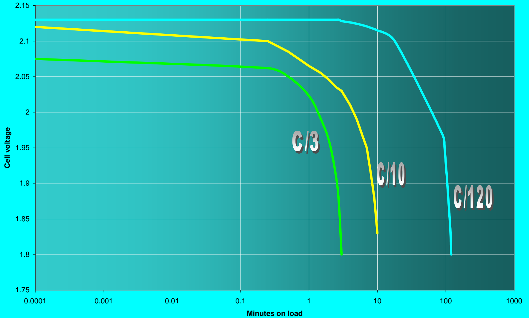
Marinegel typical discharge curves
